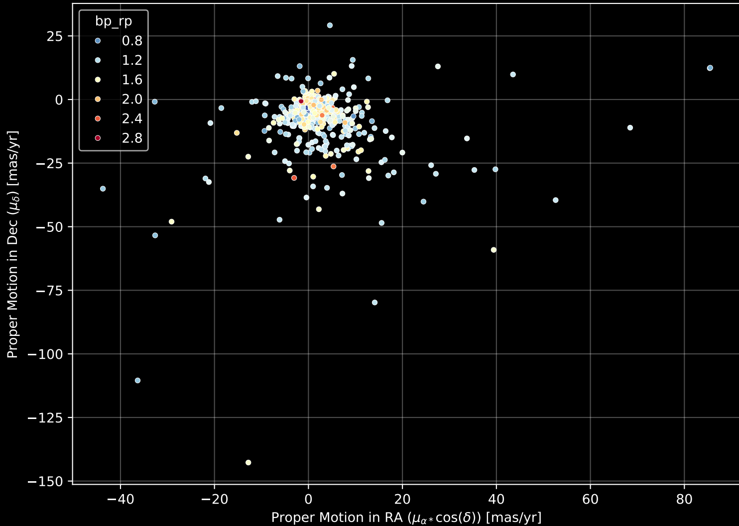
GALAH DR4 Field: [6778] Proper Motion Diagram (n= 503)
