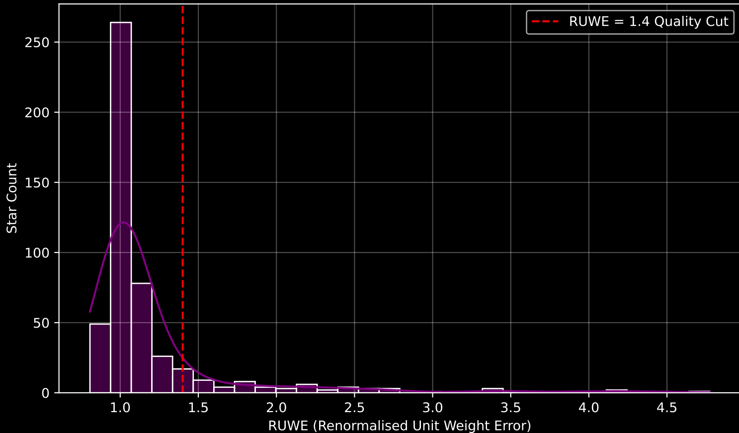
GALAH DR4 Field [6778] RUWE Distribution (n= 493)
