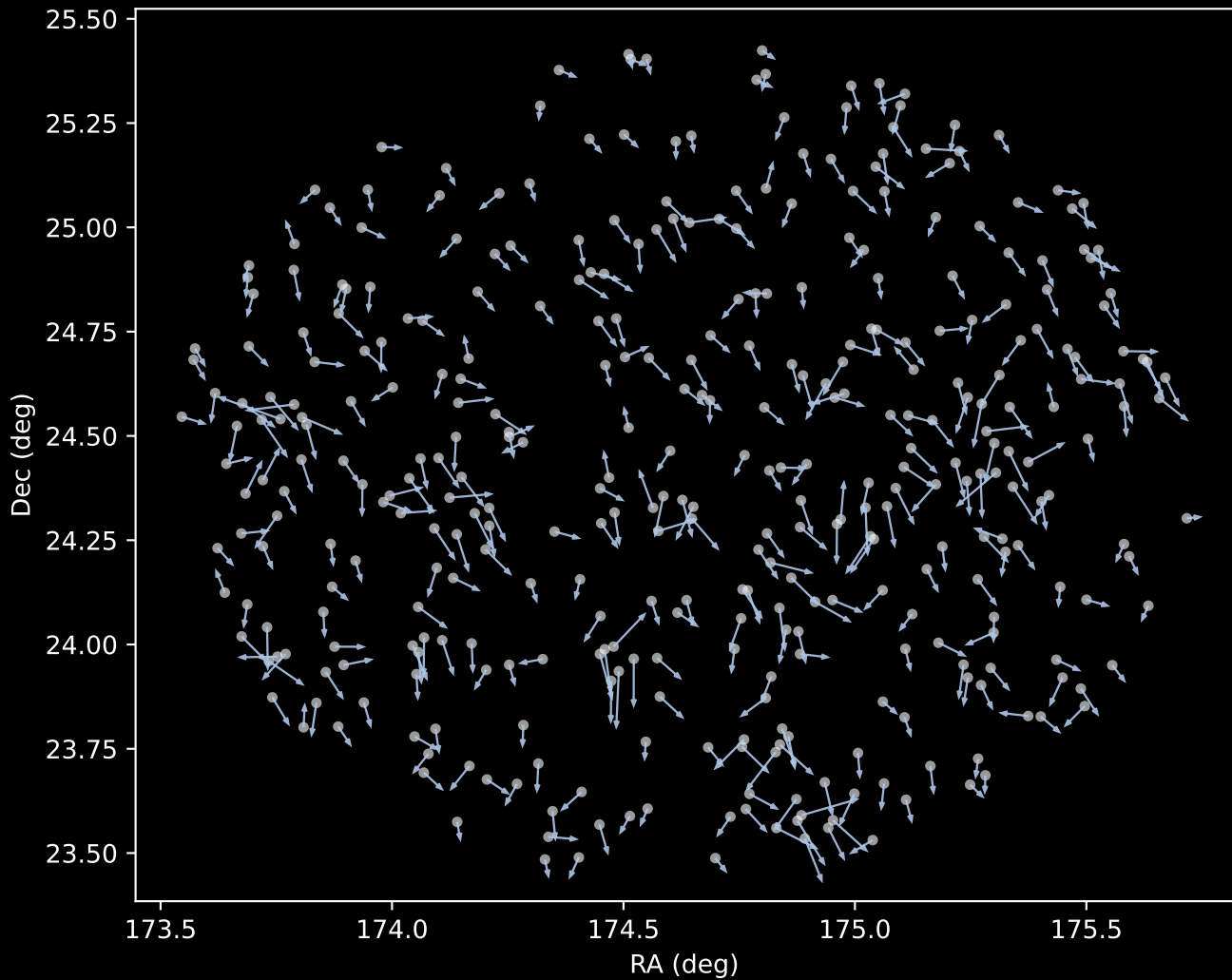
GALAH DR4 Cluster 1 Proper Motion Vectors (n=374)
